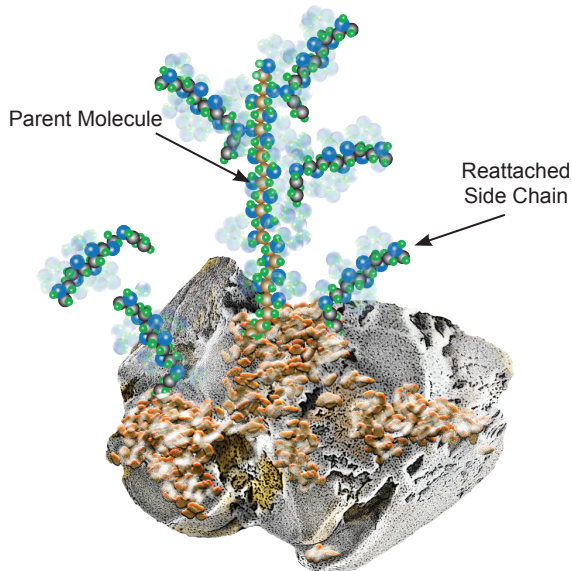
Fig. 2 Illustration showing cleavage, disassociation and reattachment of fragmented side chain surfactants on water repellent soil particle surface.
